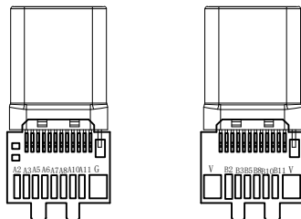
TYPE C3.1 Female welding surface
