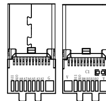
TYPE C3.1 Male welding surface
